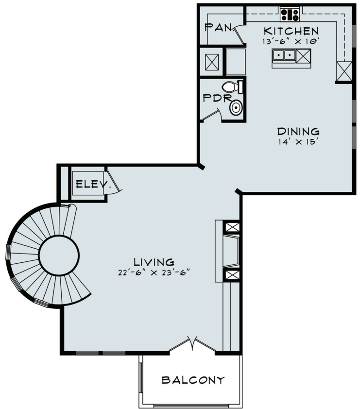
SECOND FLOOR
