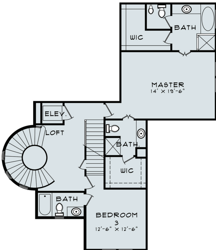
THIRD FLOOR
